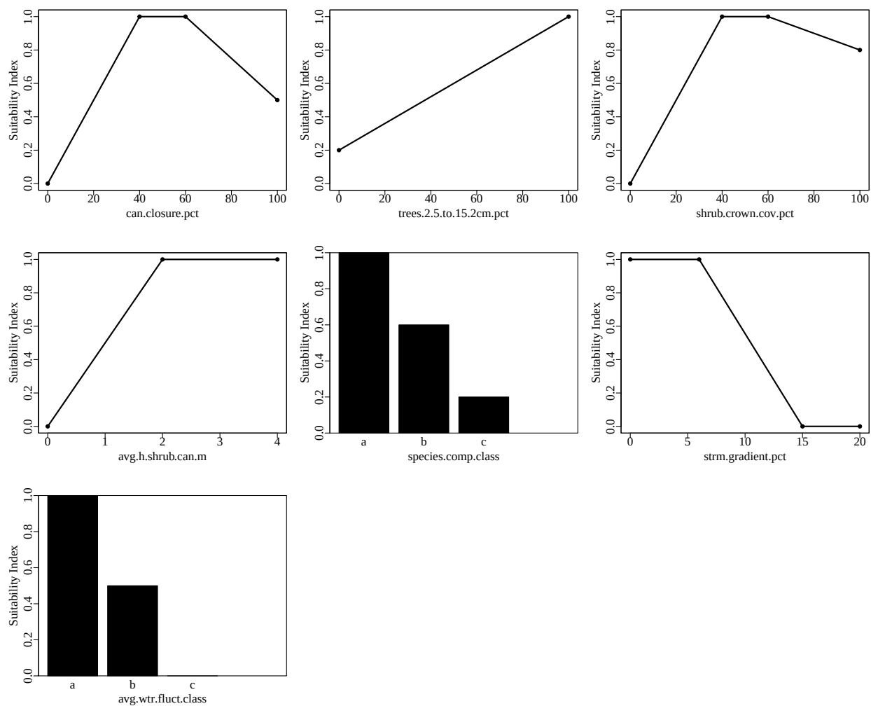
Figure 1. Suitability index graphs for variables included in the beaverRiv model in ecoest.
